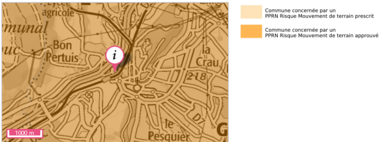
Source: BRGM
