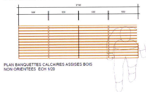
FACADE BANQUETTES CALCAIRES ASSISES BOIS NON ORIENTEES ECH 1/20
